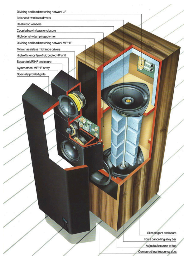
Figure 2. Reference 104/2 - the internal twin bass drivers were braced using a metal rod, allowing for a force cancelling arrangement
