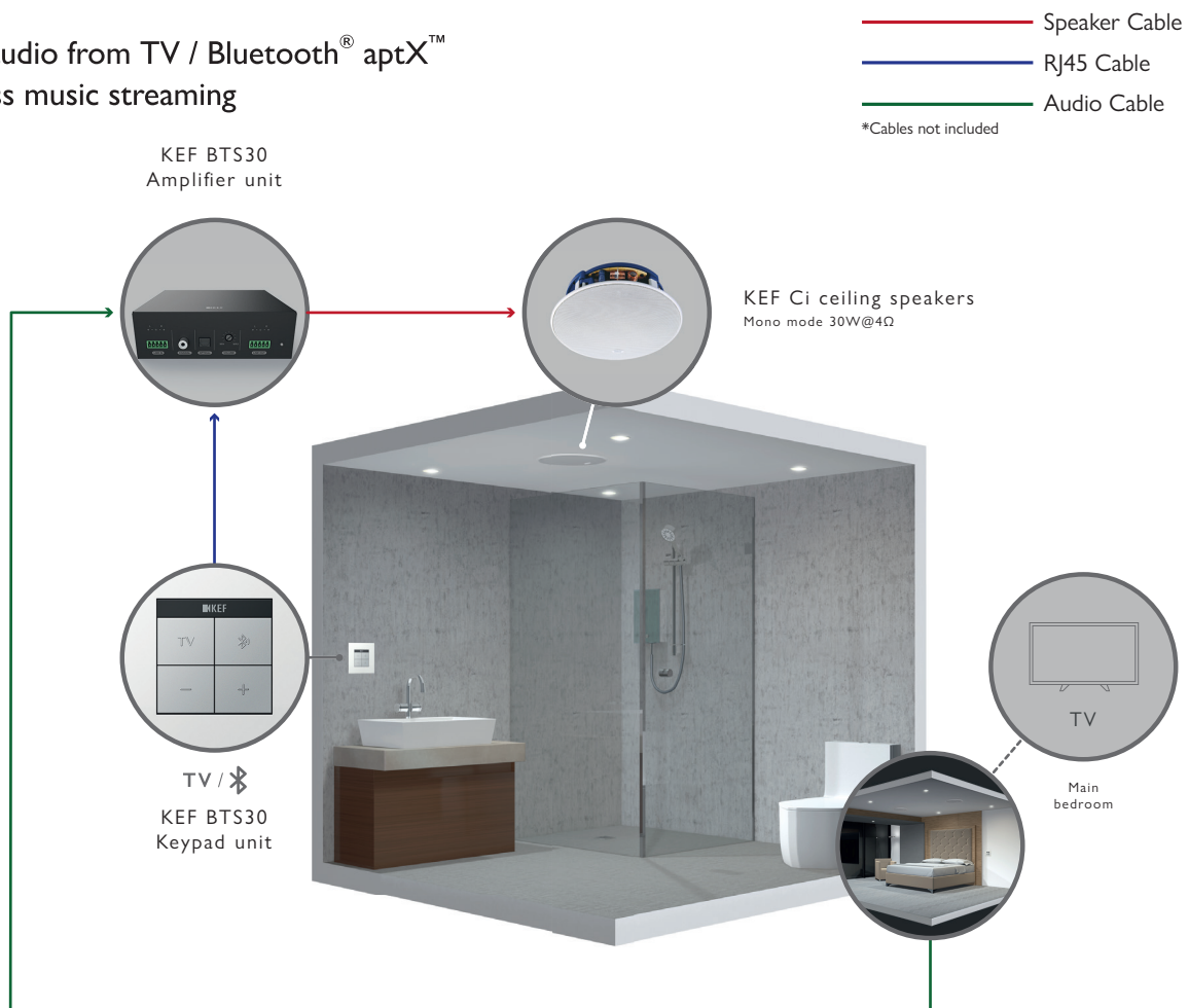
Delivering TV sound to bathroom
