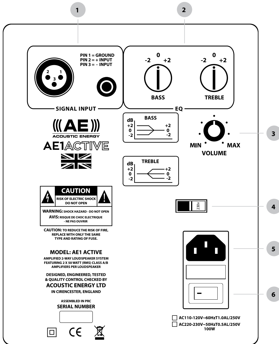
Rear connections and controls, refer to numbers and instructions opposite
